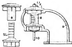
Figs. 3061-3065. Chamber's Compensating Throttle Valve.
